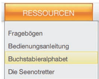
Abb. 6: IC-soft Ressourcenmenü
